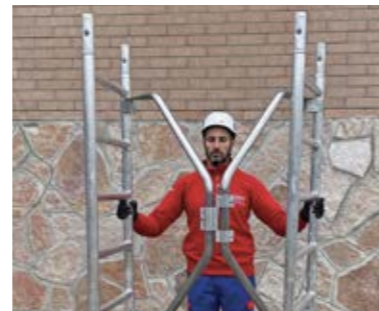
Base con kit richiudibile standard. Base with folding kit.
