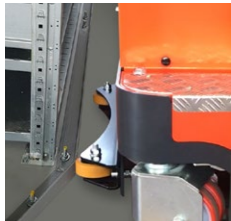
RL Side rollers
